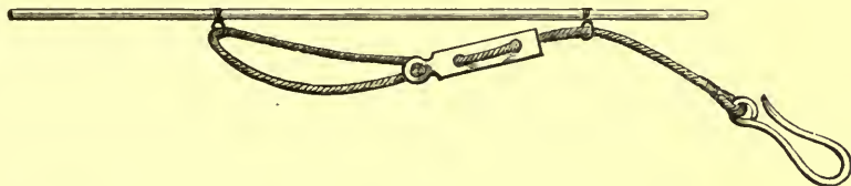
Enlarged Diagram of how to fix the sliding sheets for the respective booms, i. e. jib, fore, and main.
